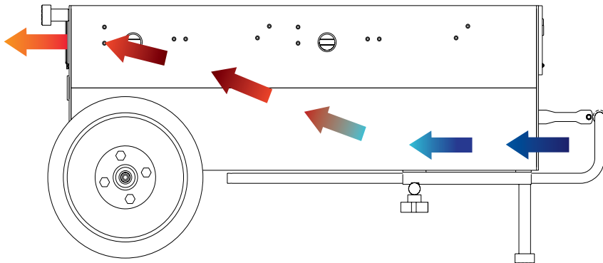
Figure 2.7.2 Horizontal Position
