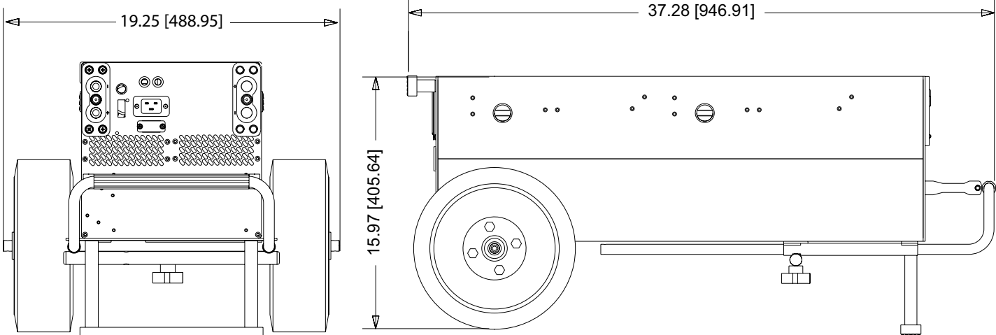
Figure 2.5.1 - TI2500 GPU-24 physical dimensions
