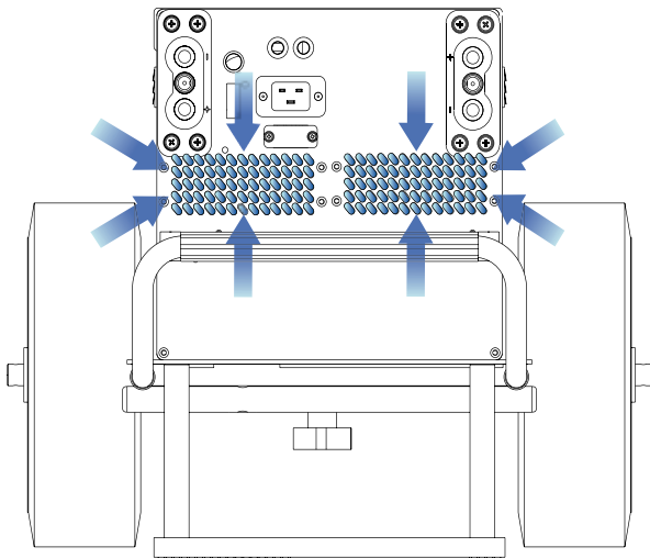
Figure 2.7.3 Front Inlet
