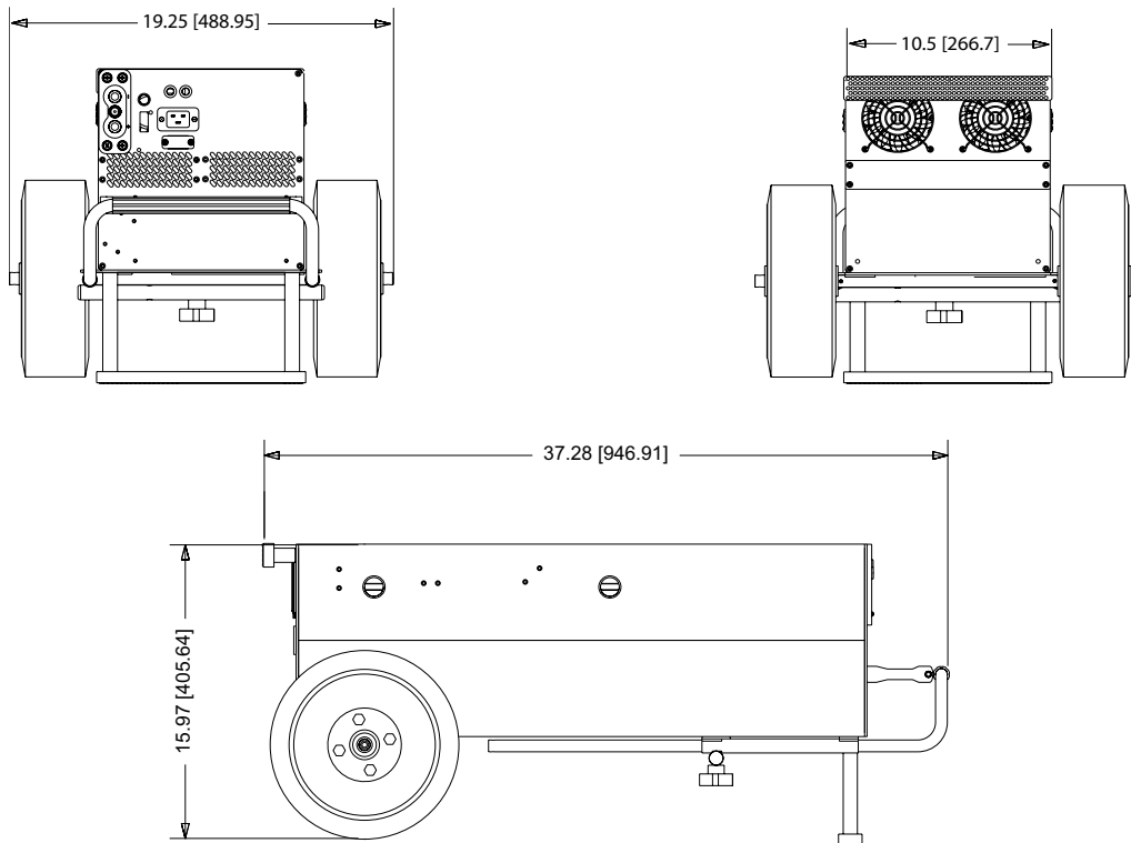
Figure 2.5.1 – TI3000 GPU-24-PFC physical dimensions
