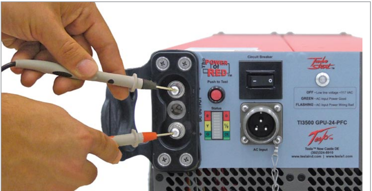
Figure 3.8.2 – Testing DC Receptacle
