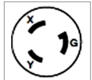
Figure 3.8.4 Schematic for Plug G is the Ground
