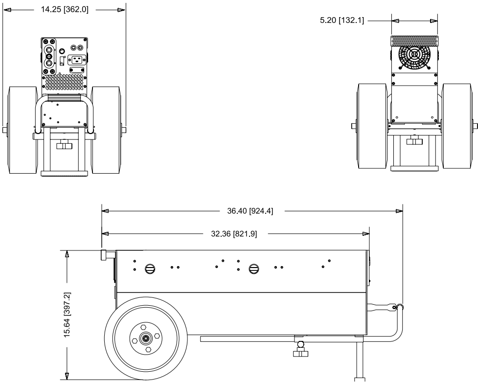
Figure 2.5.1 – TI3000 GPU-24 physical dimensions
