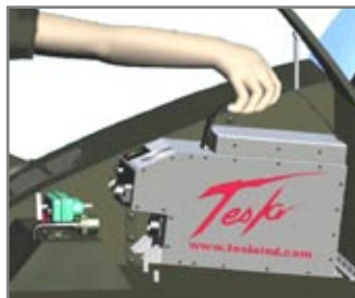
Figure 2.11.2 – Slide back flange into receiving lip
