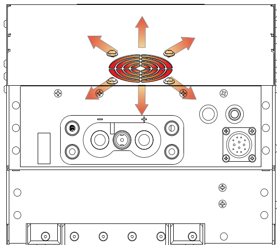
Figure 2.7.3 Front Outlet
